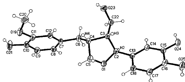
Figure 1. An ORTEP diagram showing the molecular structure of taxiresinol 1 with atomic numbering scheme. Only H atoms attached to chiral centers are numbered.
